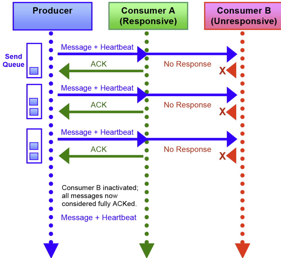
Figure 2: Slow consumer inactivated to clear send queue
