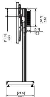
Side Elevation
