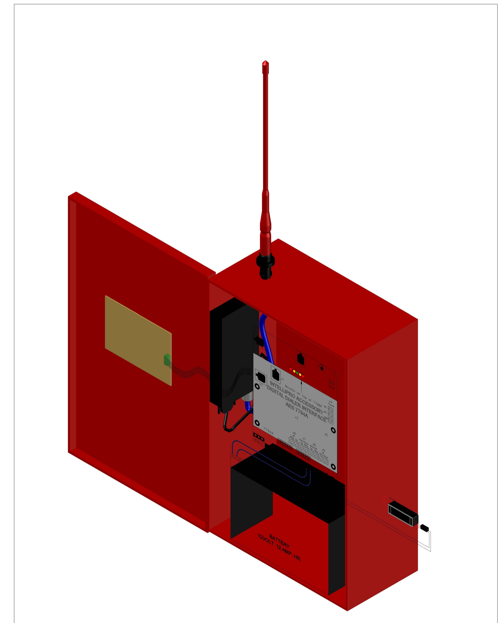
7707P-88-ULP 3D VIEW
