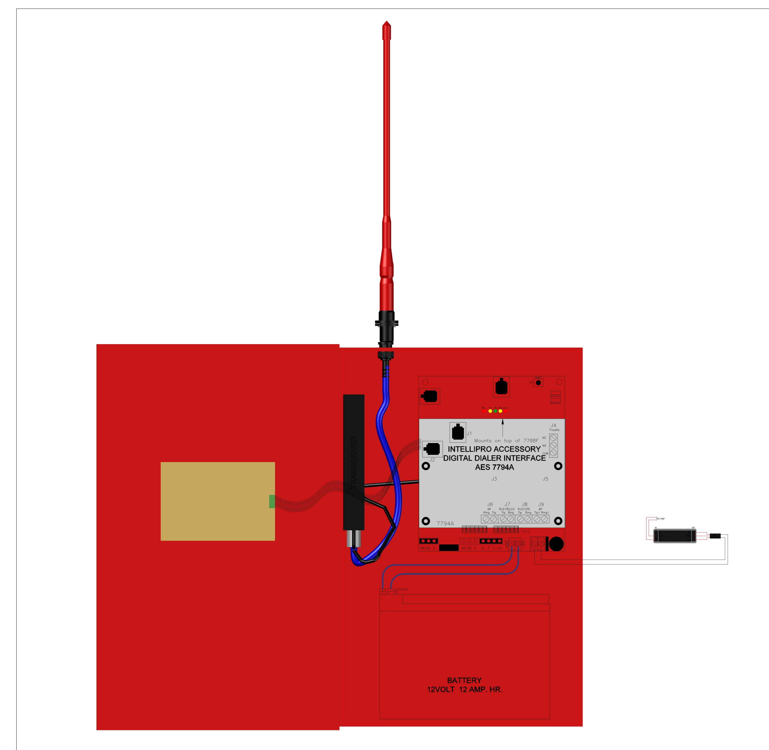
7707P-88-ULP FRONT VIEW
