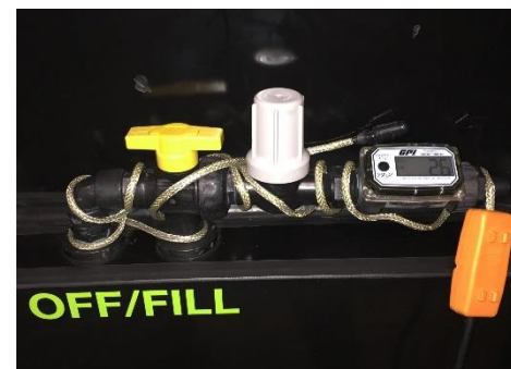
Heat Tape
