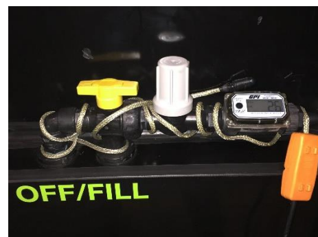
Heat Tape
