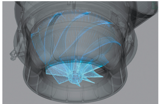
Impeller integrated in the motor bucket.
