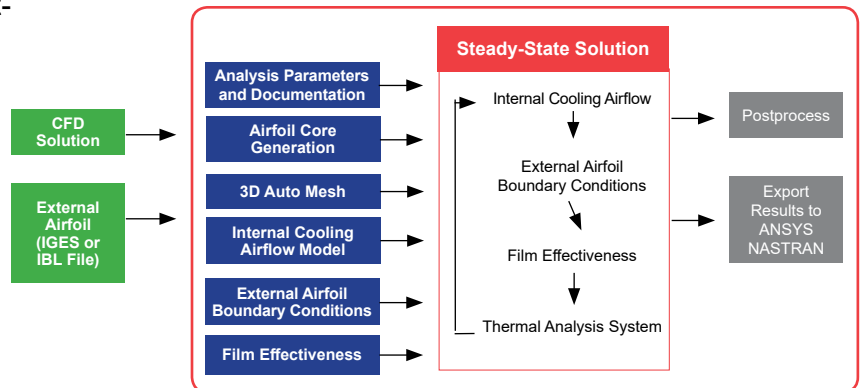
CTAADS System Schematic
