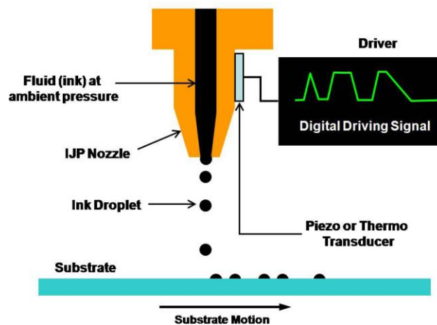
Figure 5: Piezo inkjet printing ( www.spie.org )
