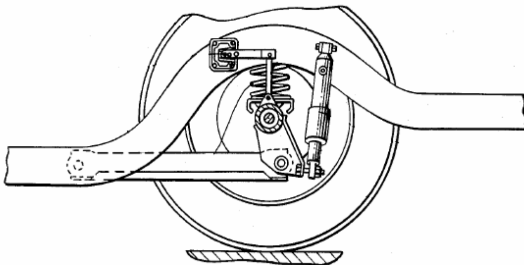
Figure 1: Side elevation view of a vehicle suspension of sprung and unsprung masses including the suspension means, shock absorber, and level sensor
