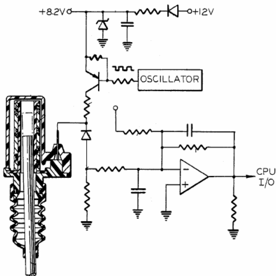
Figure 2: Alternative level sensor and circuit
