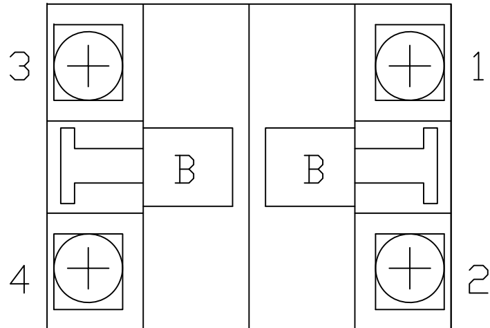
TERMINAL VIEW
