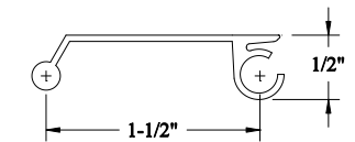
Model 6544: Extruded Aluminum Slats
