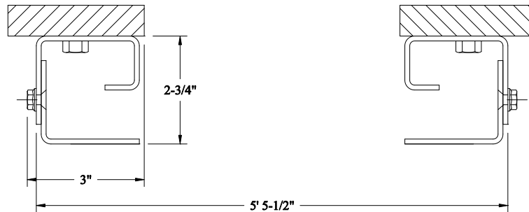
"X" DIMENSION "X" Dimension = Opening Width + 5-1/2"
