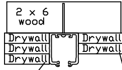
Triple Drywall Recessed track mounting Into wood header
