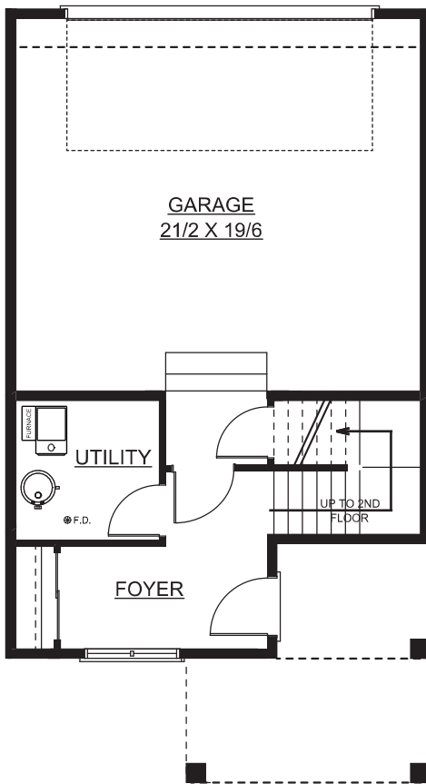
MAIN FLOOR PLAN 176 SQ. FT.
