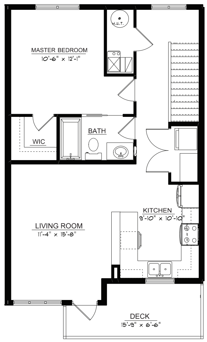
THIRD FLOOR PLAN 732 SQ. FT.
