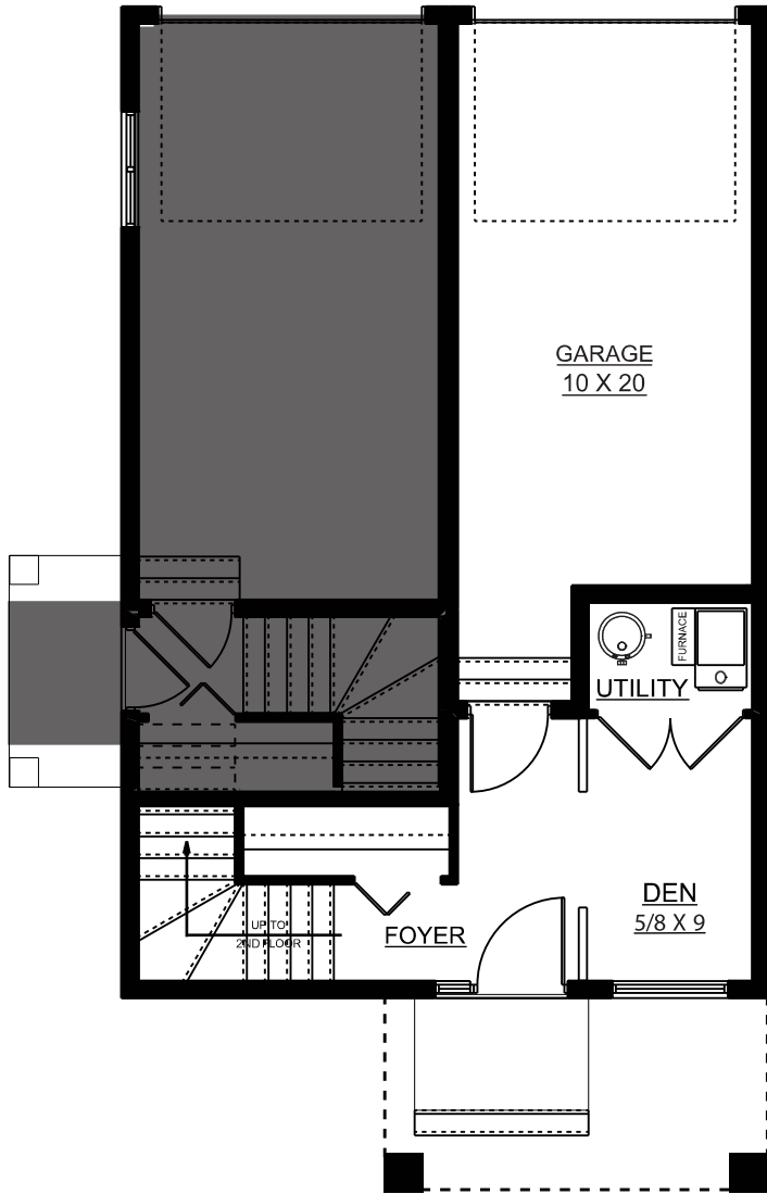
MAIN FLOOR PLAN 210 SQ. FT.
