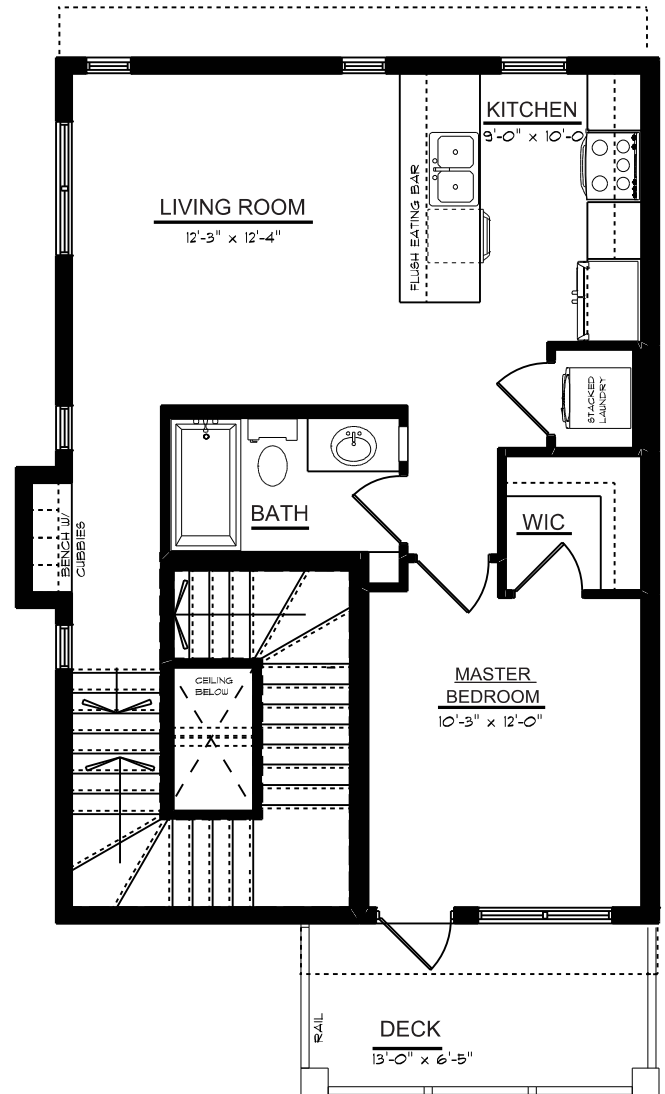
SECOND FLOOR PLAN 590 SQ. FT.
