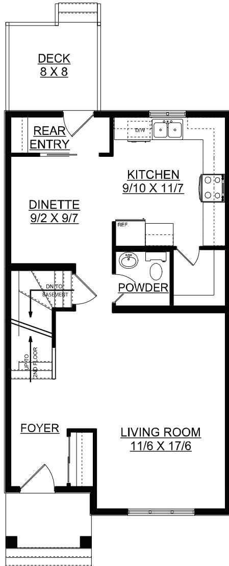
MAIN FLOOR PLAN 693 SQ.FT.
