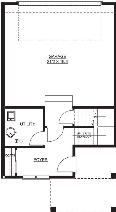
ENTRY PLAN 176 SQ. FT.
