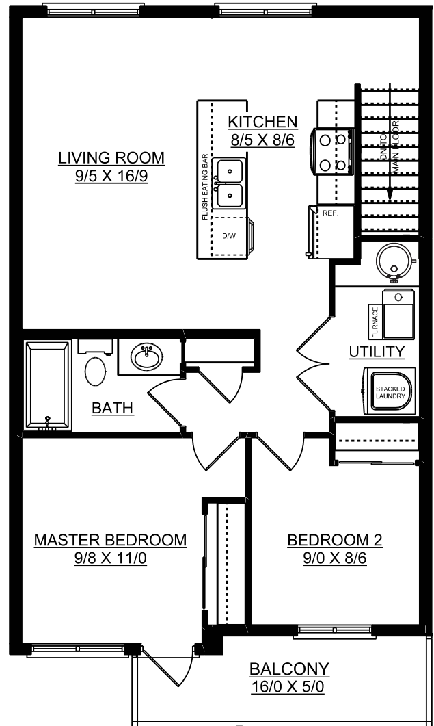
SECOND FLOOR PLAN 749 SQ. FT.
