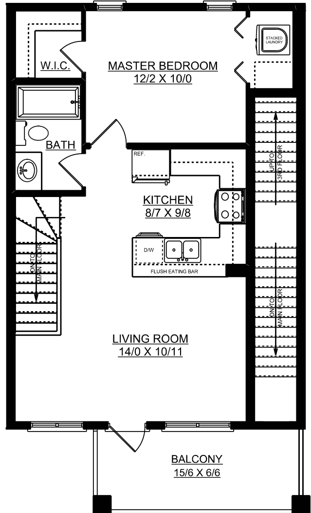
SECOND FLOOR PLAN 611 SQ. FT.
