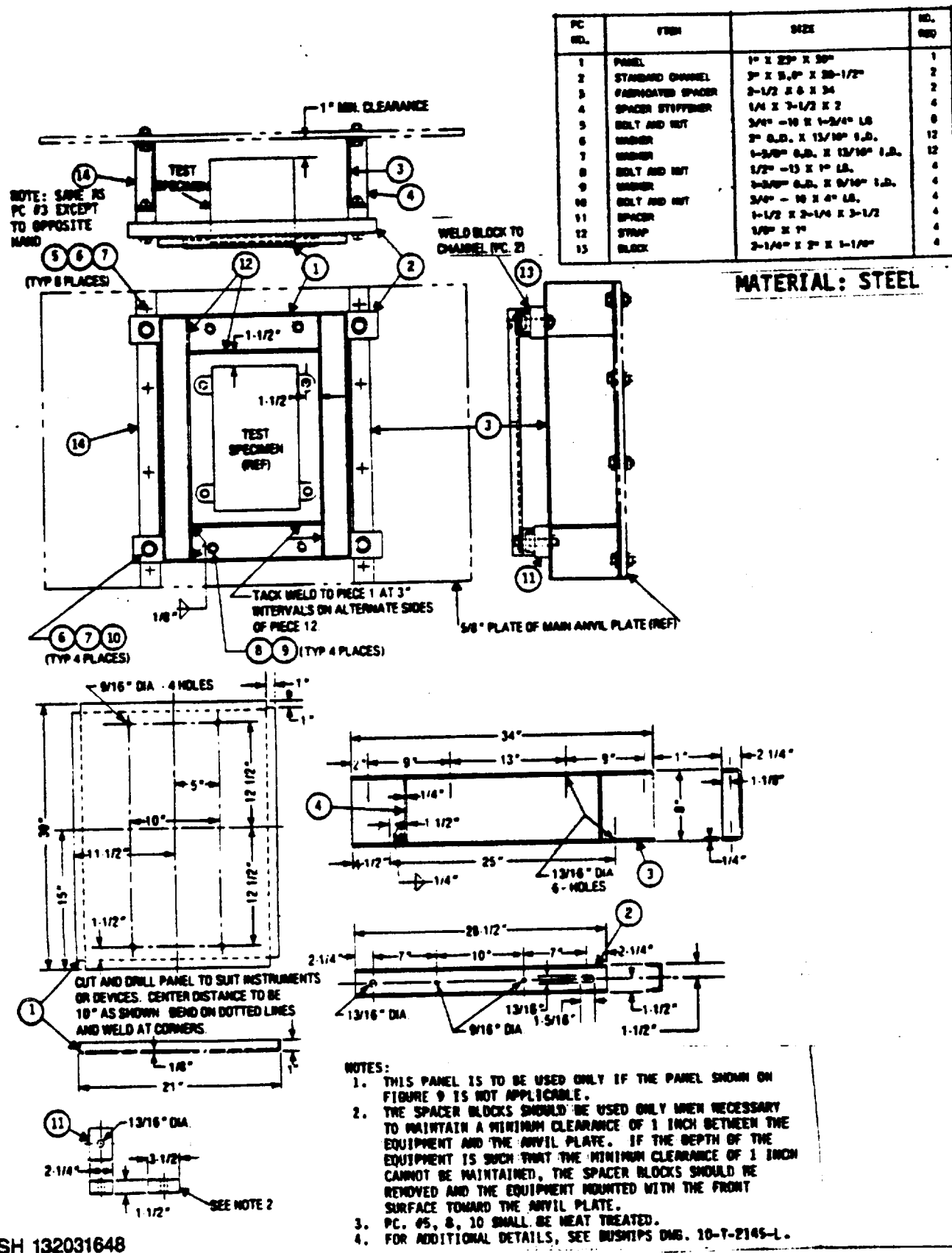
FIGURE 10. Fixture 8D-2 standard mounting for electrical indicating switchboard meters and other panel mounted equipment (type "C" test LWSM).
