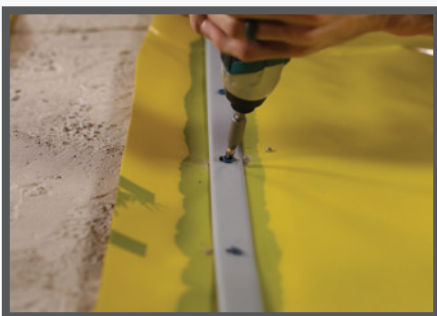
Onto a Perimeter Footing at Impediments: Seal Stego Wrap to concrete with Stego Mastic.
