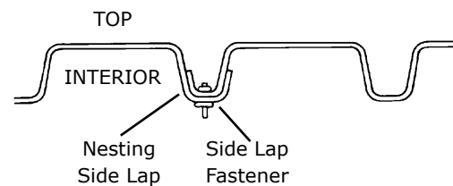
Roof Deck Side Lap Detail
