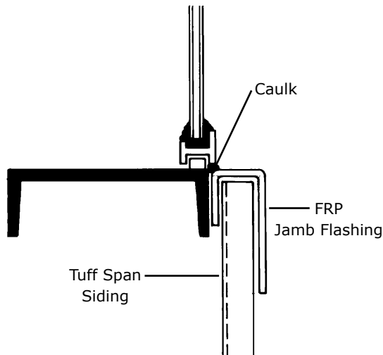
Sill Detail
