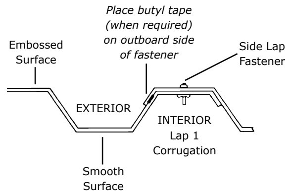
Roof Deck Side Lap Detail
