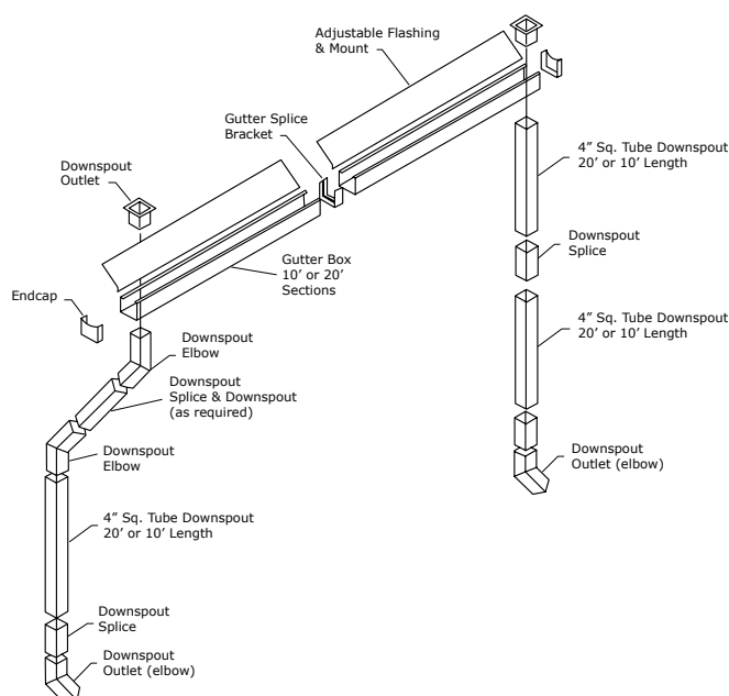
Tuff Span gutter, downspout, roofing, and siding at metal alloy processing plant
