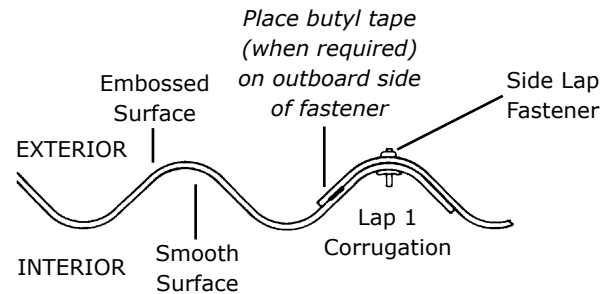
Corrugated Panel Side Lap Detail
