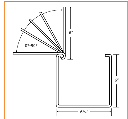
Hinged gutter flange pivots to match any roof slope.
