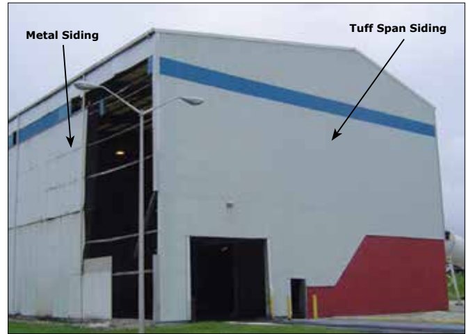
At Waste to Energy facility, Tuff Span roofing and siding (on end wall) were undamaged by Hurricane Charlie's 145 mph winds. Corroded metal panels (on side wall) were damaged or blew off.
