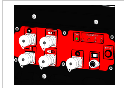
Drives up to 4 shafts, depending on the version: wire feed, AVC, OSC and wire
