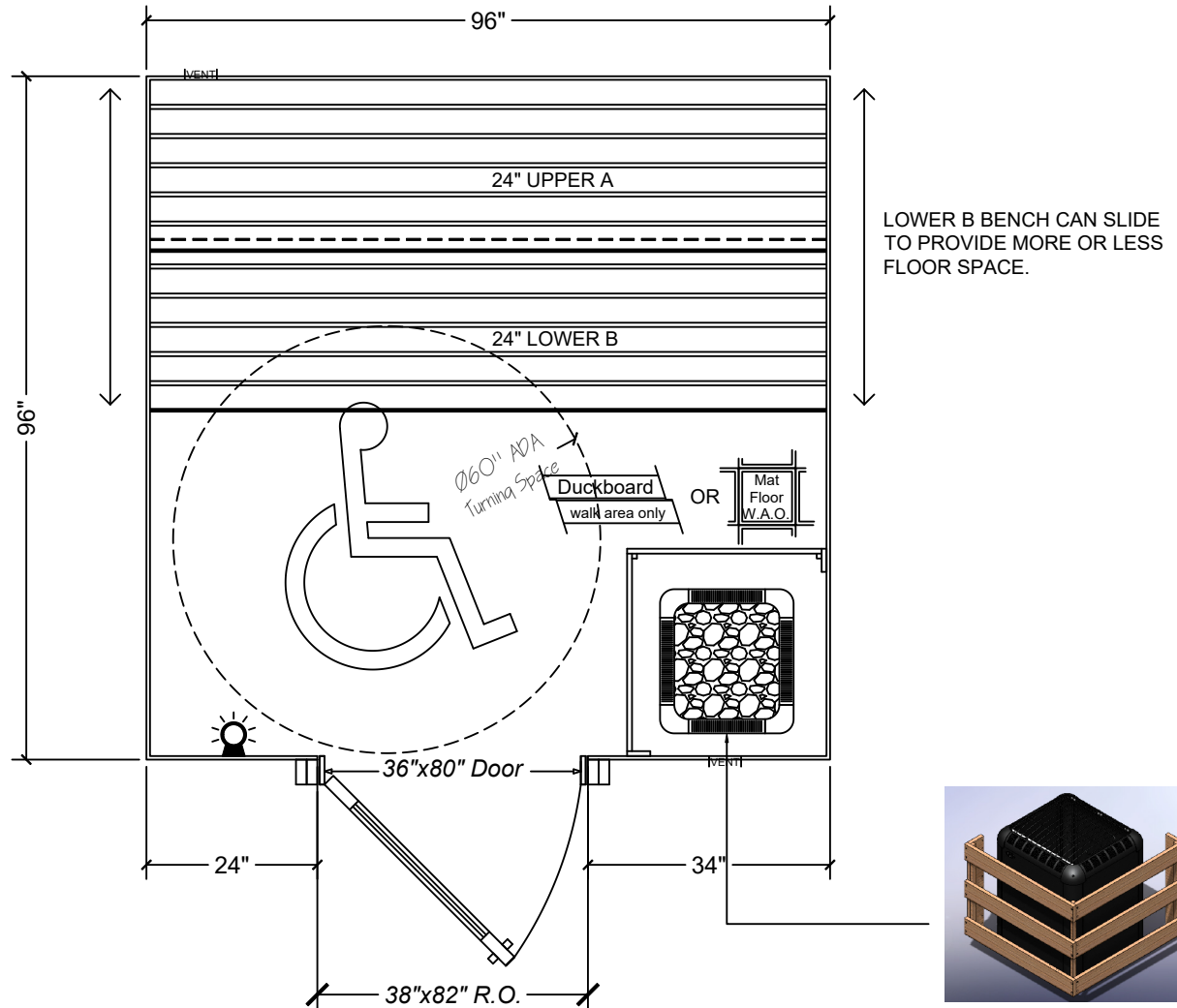
Laava Heater: As shown in CAD below
