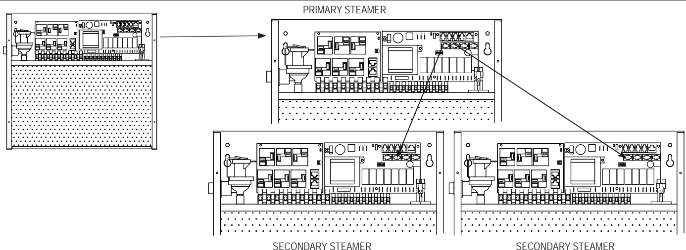
DIAGRAM 9: CONNECTING STEAMERS
