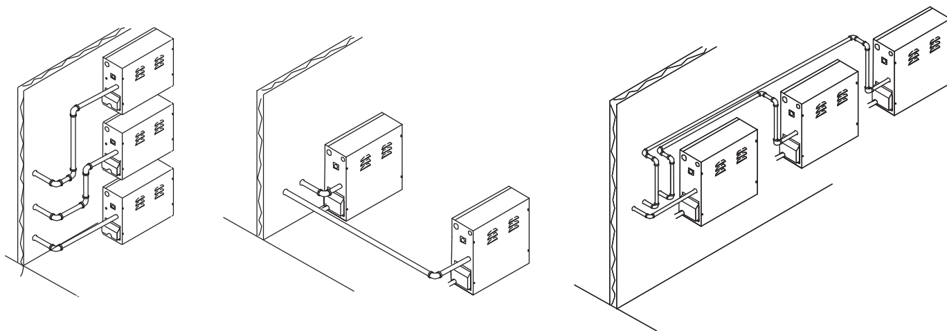
DIAGRAM 7: TYPICAL STEAM LINES
