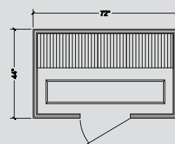
B 880-C Series 4-person
