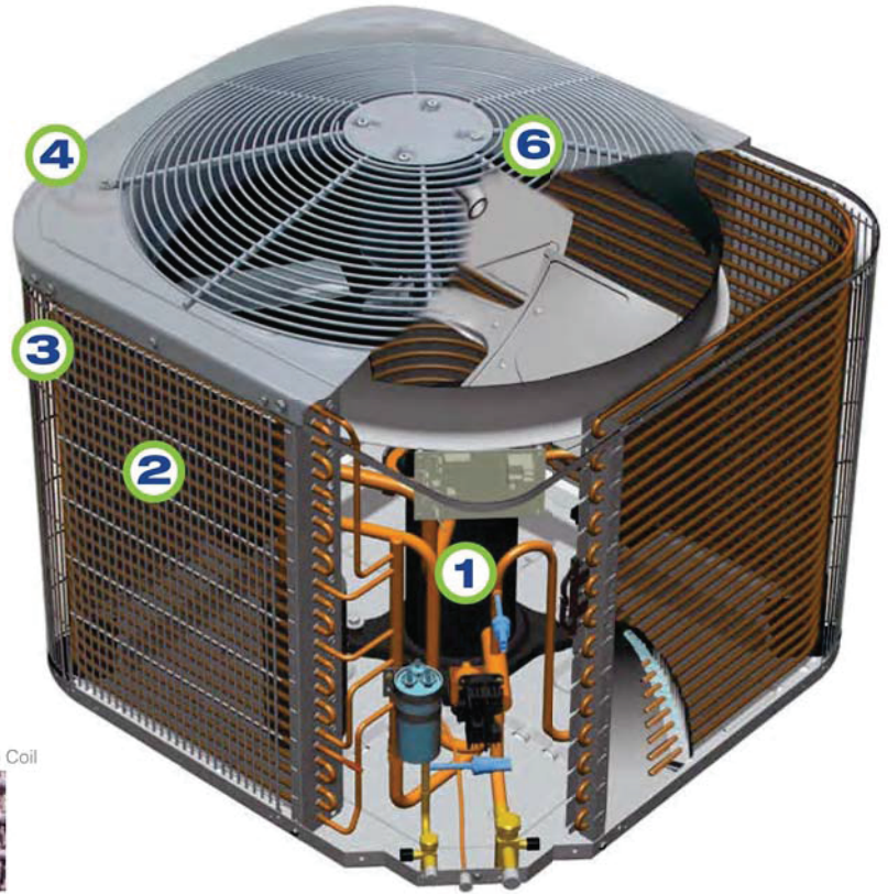
Carrier™ Series "Coastal" Heat Pump Coil with ArmorPlate™ Coating
