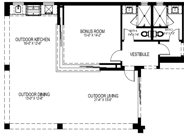
BONUS ROOM, BATHS AND OUTDOOR OPTION
