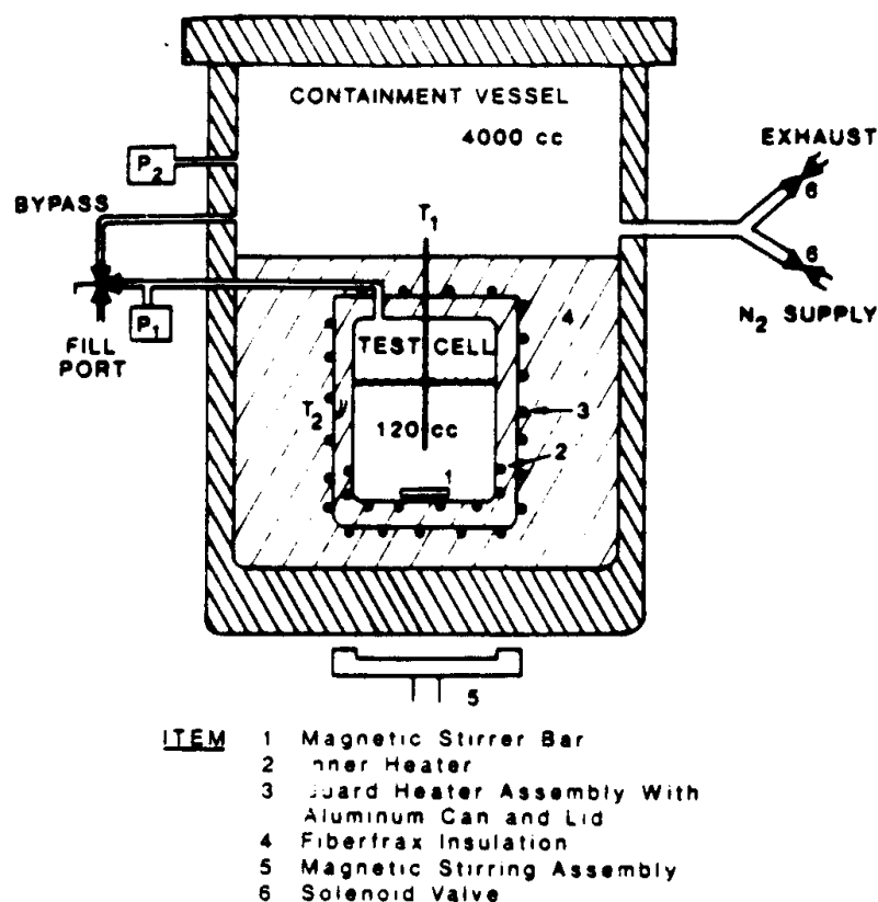
Fig. 1. Bench-scale test apparatus.
