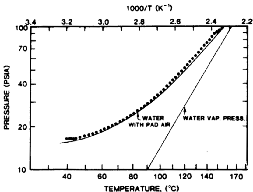
Fig. 11. Pressure-temperature data from base-catalyzed phenol-formaldehyde reaction.
