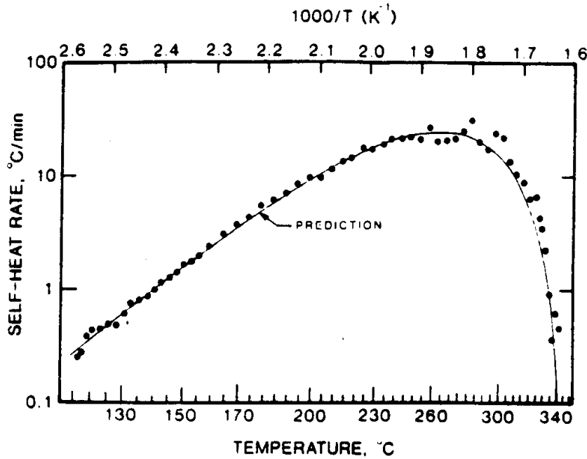
Fig. 3. Self-heat rate data from styrene runaway polymerization.
