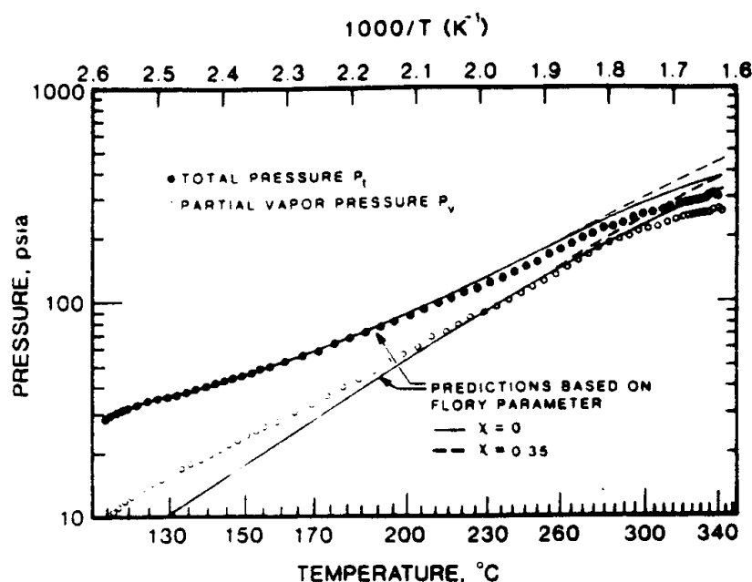
Fig. 5. Pressure-temperature data from styrene runaway polymerization.
