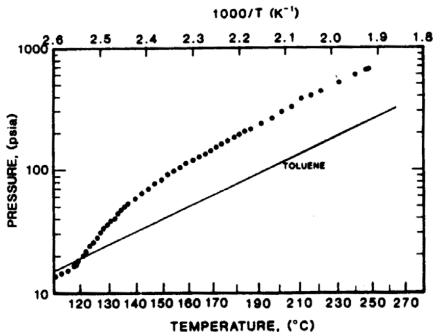
Fig. 8. Pressure-temperature data from di-t-butyl peroxide decomposition.
