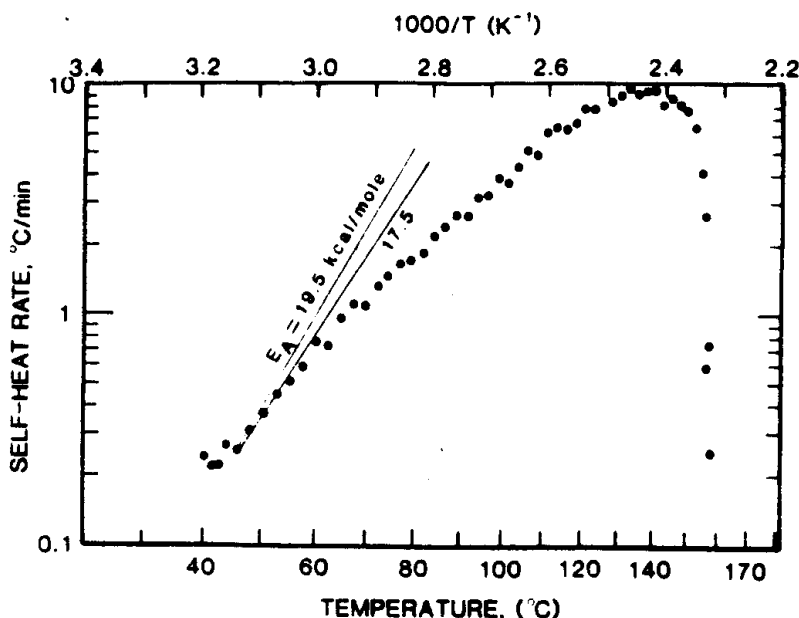
Fig. 10. Self-heat rate data from base-catalyzed phenol-formaldehyde reaction.
