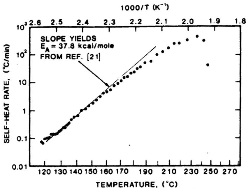
Fig. 7. Self-heat rate data from di-t-butyl peroxide decomposition.
