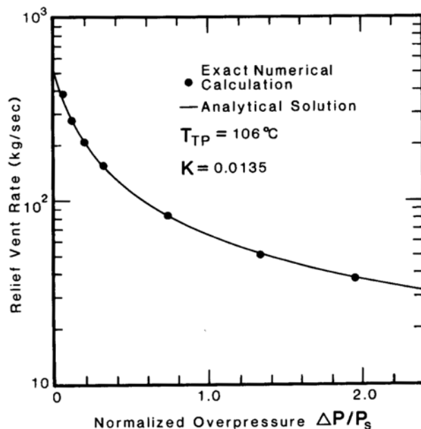
Figure 5. Relief vent rate vs. normalized overpressure.
