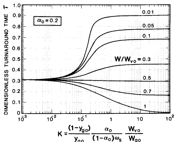
Figure 3. Generalized presentation of dimensionless turnaround time.
