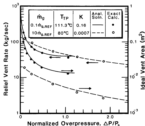
Figure 9. Additional comparison from parametric study.
