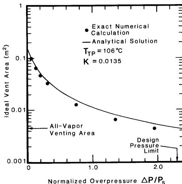
Figure 8. Vent area prediction vs. normalized overpressure.
