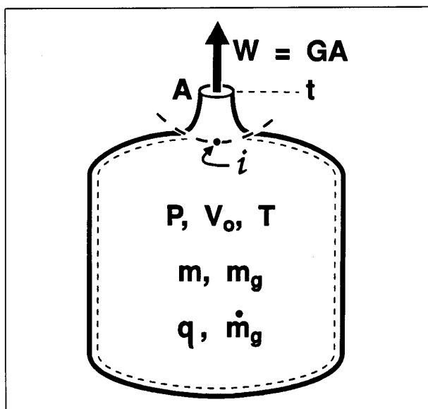
Figure 1. Reference reactor for model development.
