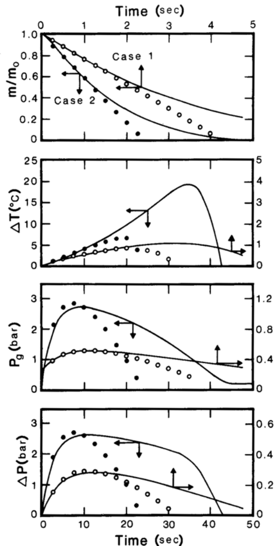
Figure 6. Venting behavior: analytical results (●, ○) vs. exact numerical solutions (—).
