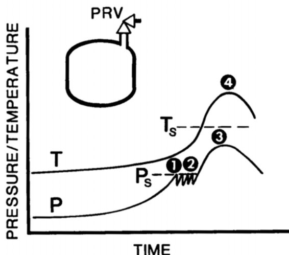
Figure 4. Venting scenario for a hybrid reaction system.
