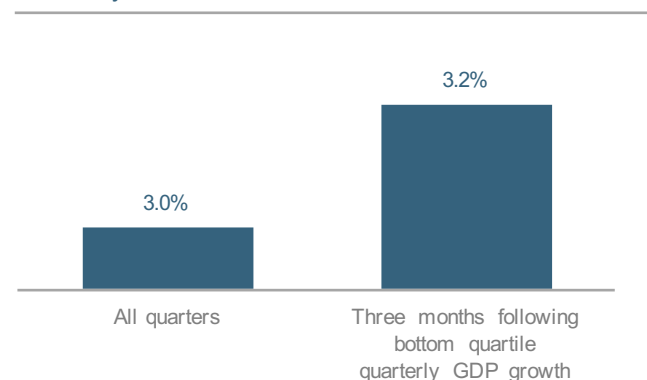
Quarterly S&P 500 Index Returns, 1948–2016
