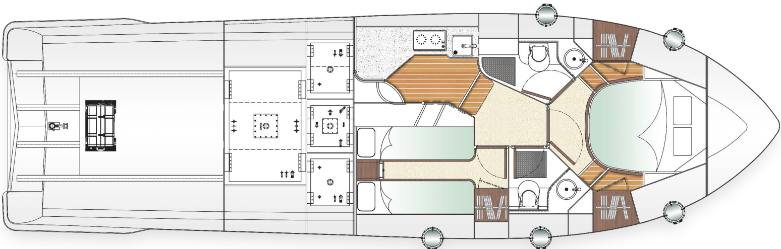
LOWER DECK
