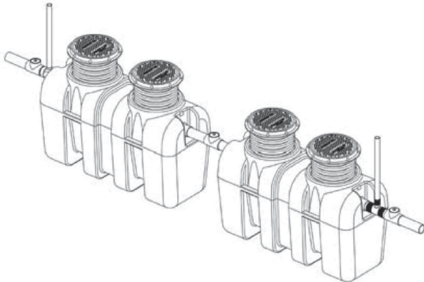
Twin units (same size) installed in-line
