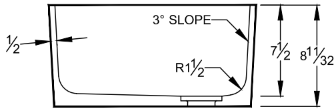
SECTION VIEW
