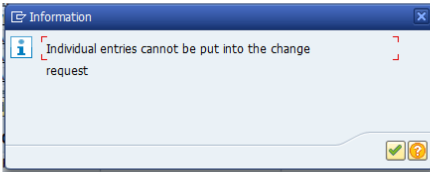
Figure 8: Information Popup
