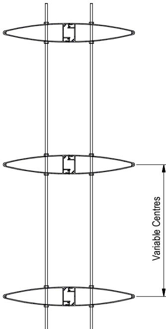
SECTIONED VIEW
