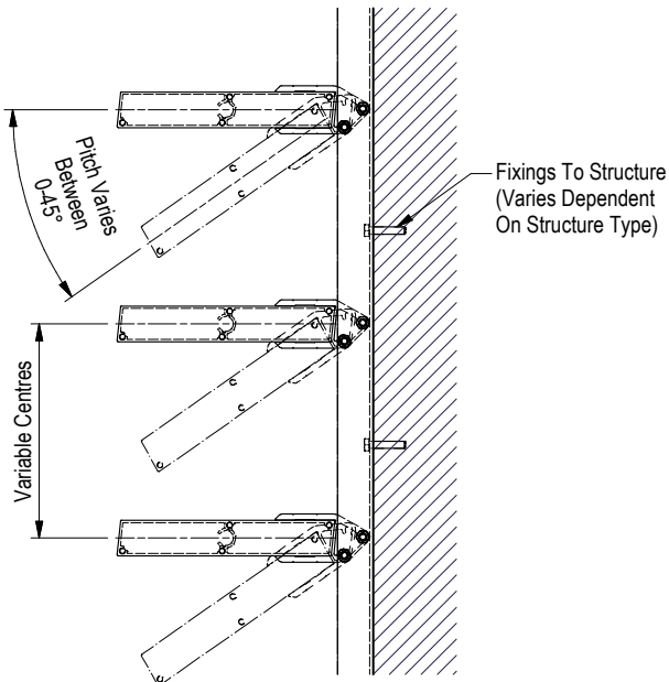
SECTIONED VIEW
