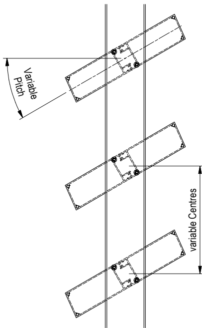
END FIXING DETAIL
