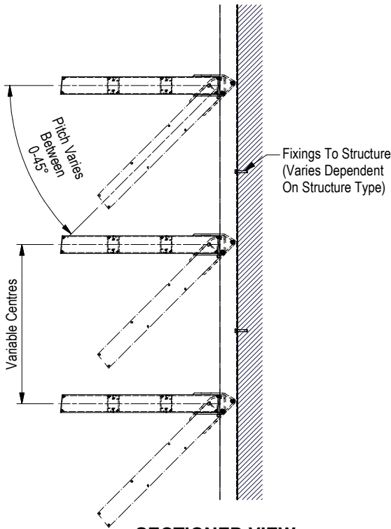
SECTIONED VIEW
