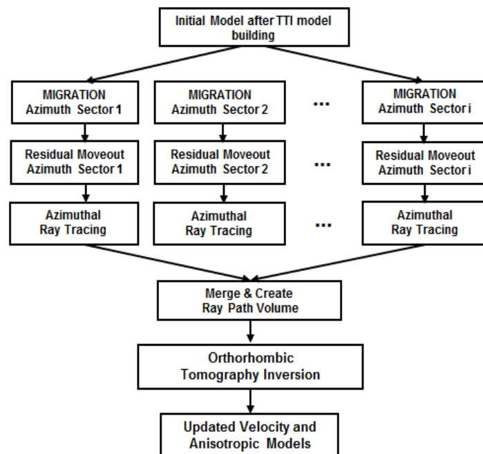
Figure 1 The workflow for orthorhombic model building.
