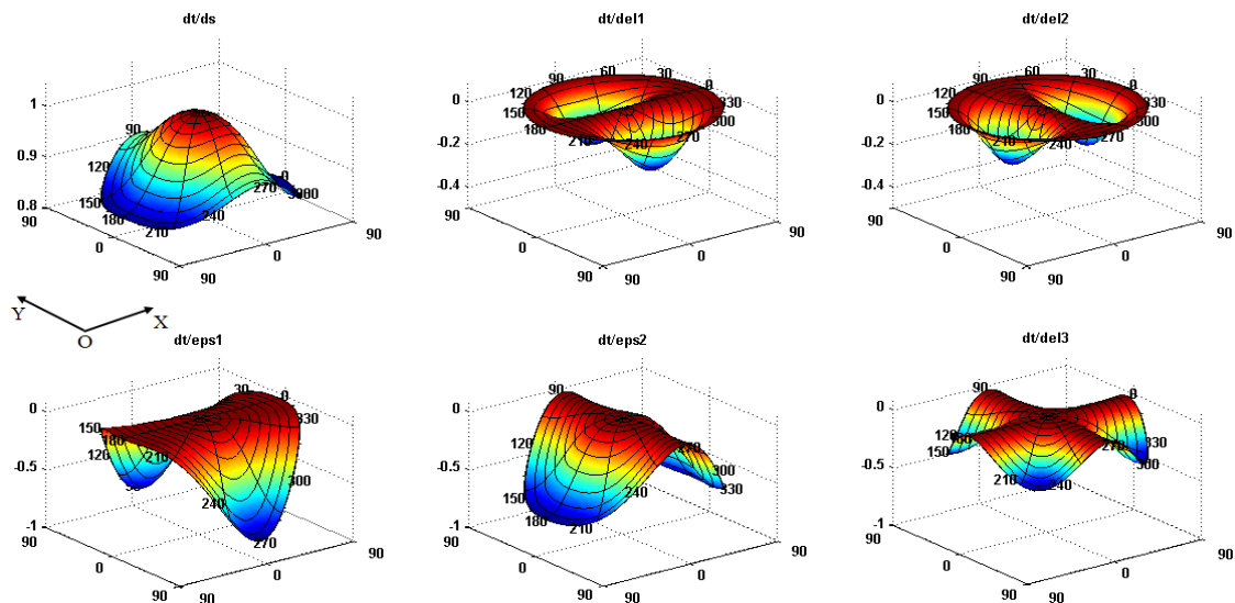
Figure 2 The derivatives of orthorhombic parameters for \epsilon^{(1)}=0.1 , \epsilon^{(2)}=0.2 , \delta^{(1)}=0.06 , \delta^{(2)}=0.12 , \delta^{(3)}=0.05 . Vertical axis represents the value of the derivatives. Azimuths are plotted from 0 to 360° with an interval of 30°. Polar angles are plotted from 0 to 90°.
