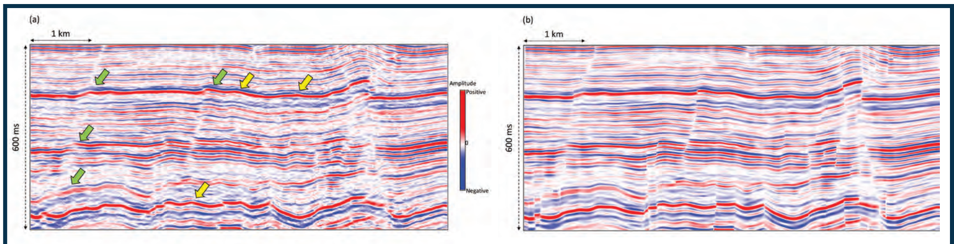
Figure 1: Vertical slices through the seismic amplitude volume (a) before and after (b) two passes of Kuwahara structure-oriented filtering. Notice how cross-cutting noise inconsistent with structural dip is suppressed, amplitudes consistent with structural dip are preserved, while discontinuities are sharpened with filtering. Green arrows indicate the footwall of a fault, while yellow arrows indicate folds that may be associated with pop-up features. Size of analysis window is 5 traces by 11 2-ms samples. (Data courtesy: Arcis Seismic Solutions, TGS, Calgary, Canada)
