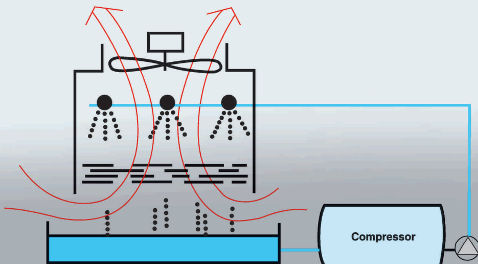
Open cooling system with circulating cooling water.
