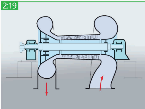
Axial compressor.
