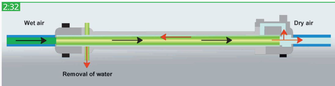
Working principle of membrane dryers.
