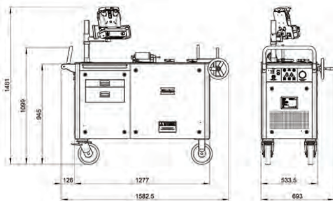
STbench Standard - Large frame dimensions
