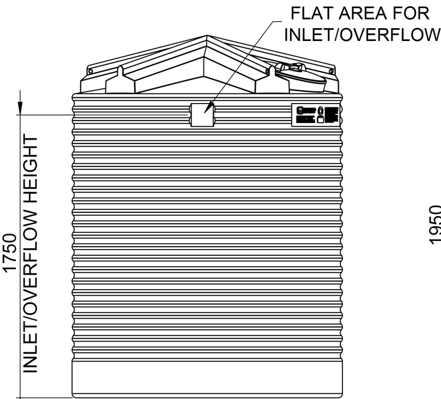
3 O'CLOCK VIEW
