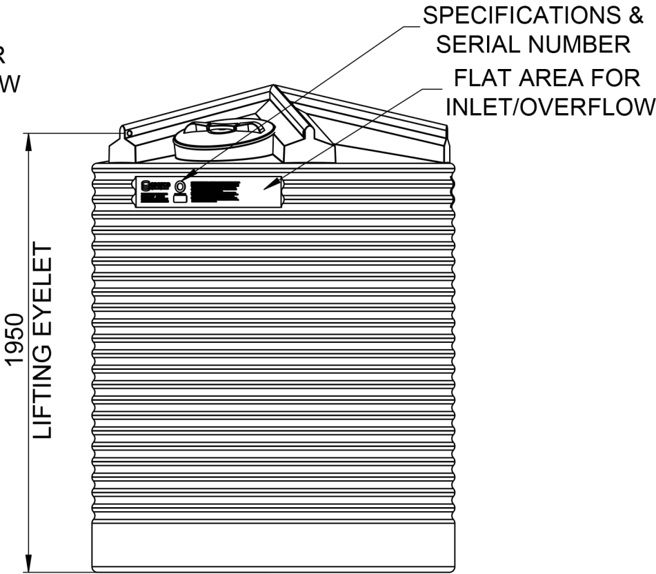
12 O'CLOCK VIEW
