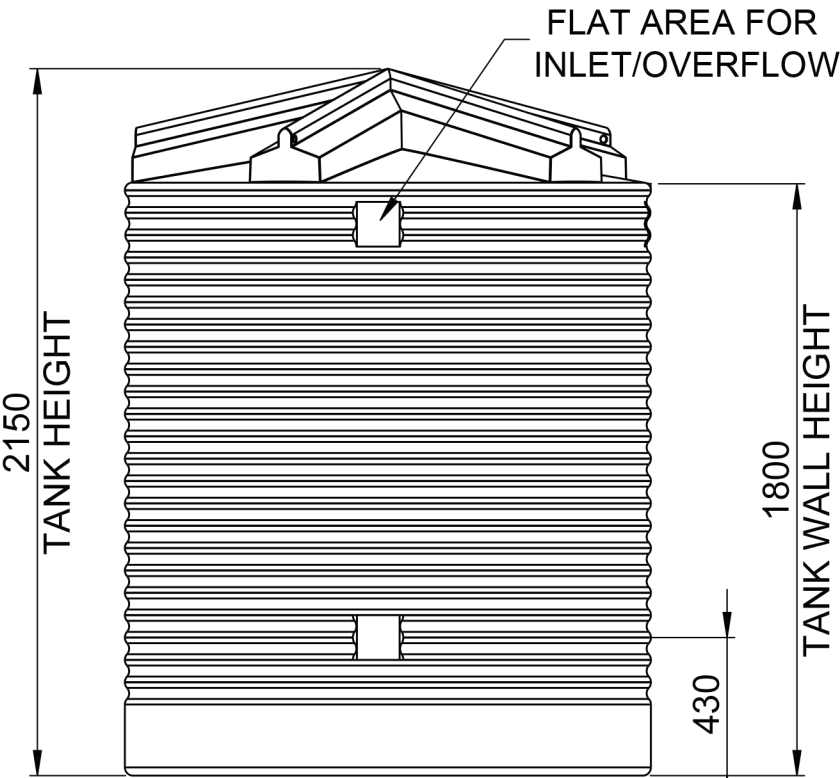
6 O'CLOCK VIEW
