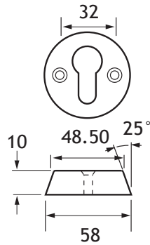
Euro Profile Escutcheon
