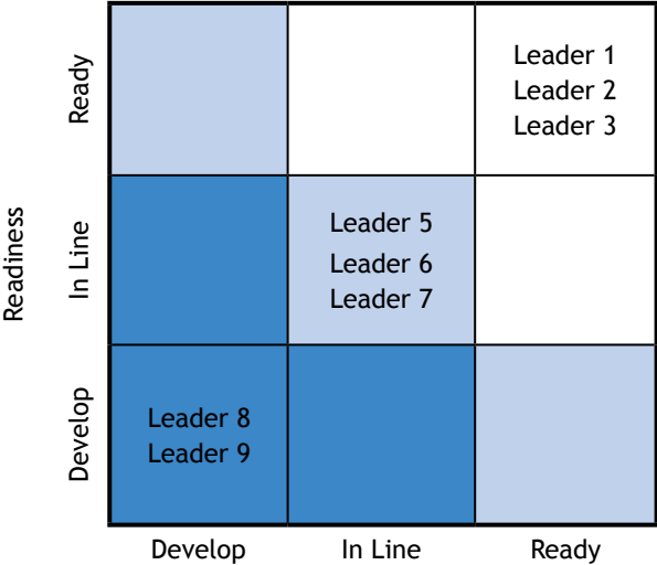
Figure 4: Ranked Board Member Readiness (All Members)
