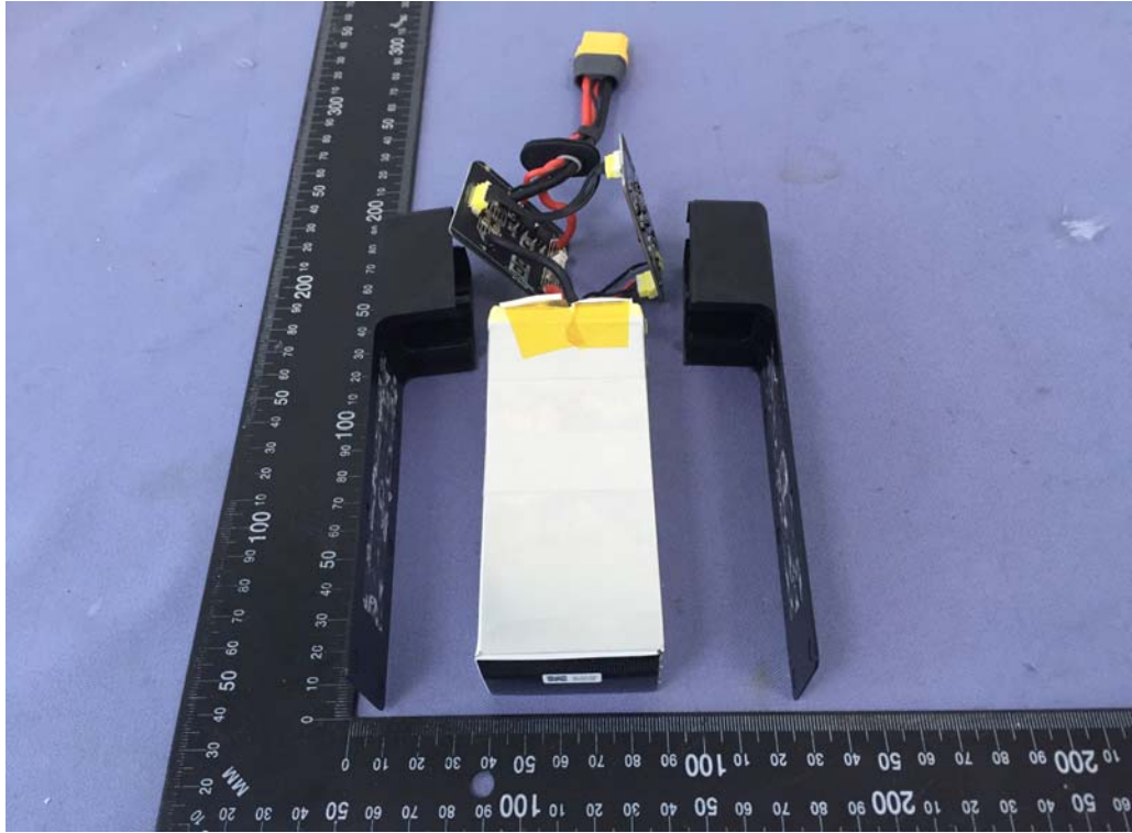
Figure 3 Internal view of battery (内部图)
