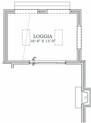
Loggia w/ Vaulted Ceiling (6a) (Skylights Optional)
