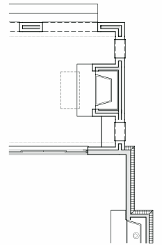
with Outdoor Fireplace (6b)
