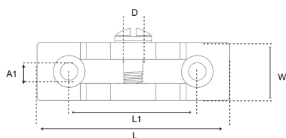
Deck Hinge 90°
