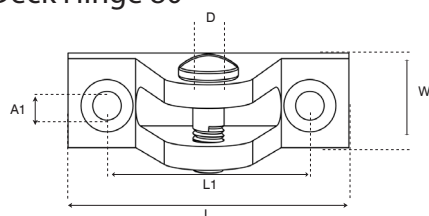
Deck Hinge 80°
