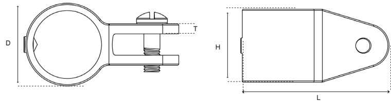
Top Slide (1 Screw)
