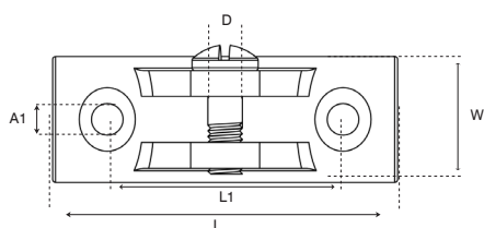
Concaved Deck Hinge
